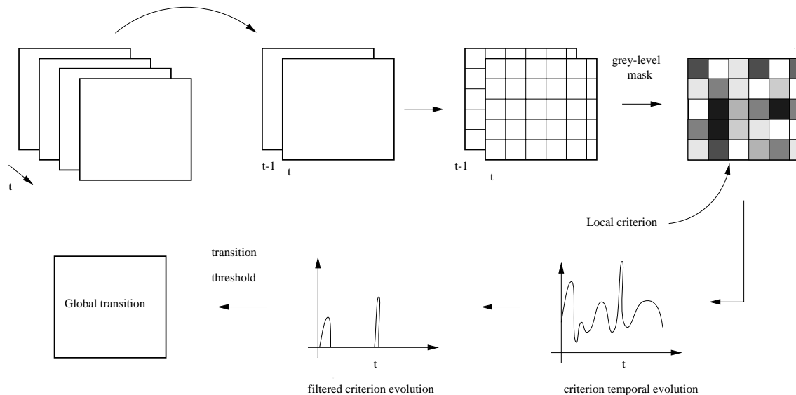
Figure 1: Description of the local algorithm.
