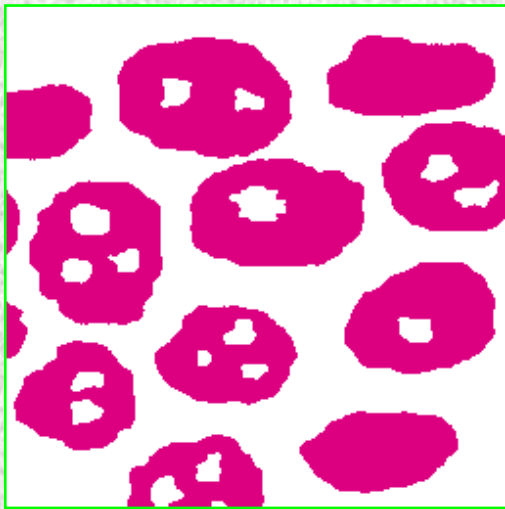
Image initiale X
