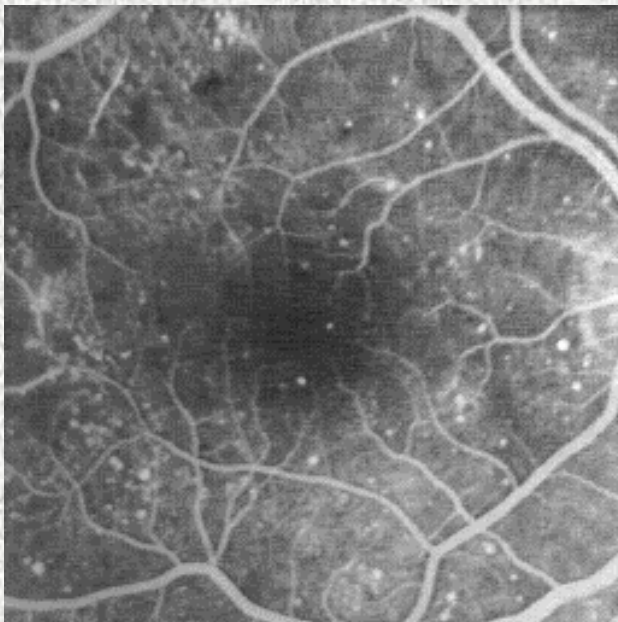
Image initiale
