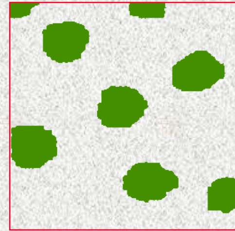
Reconstruction
