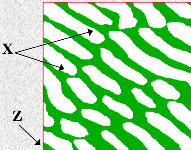
Image initiale
