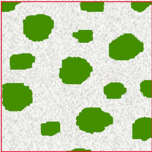
Image initiale
