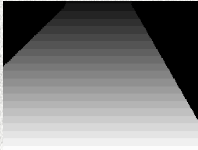
Scale factor used to define the refringence field
