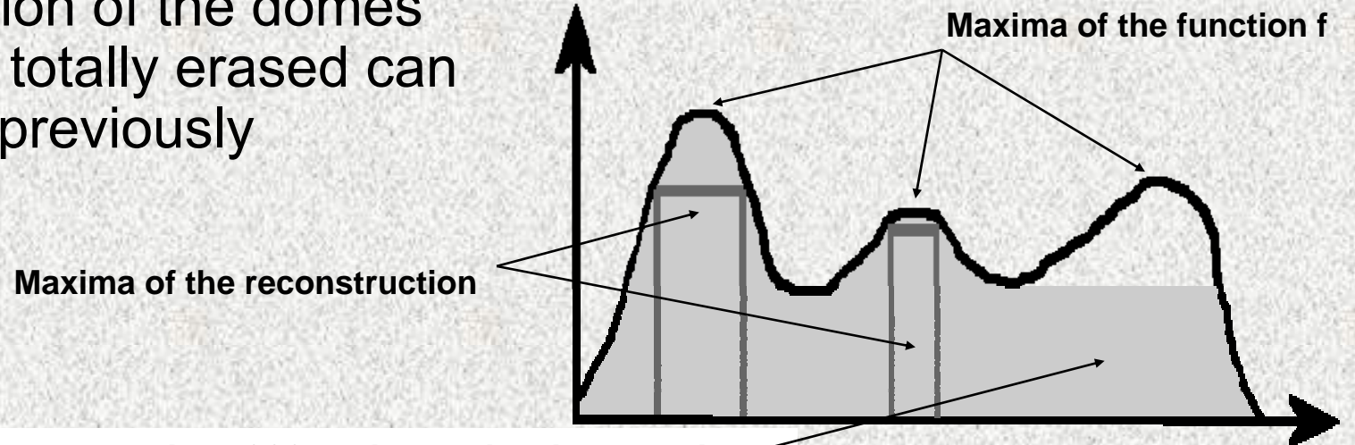
Reconstruction of f from its maxima included in the maxima of the previous reconstruction
